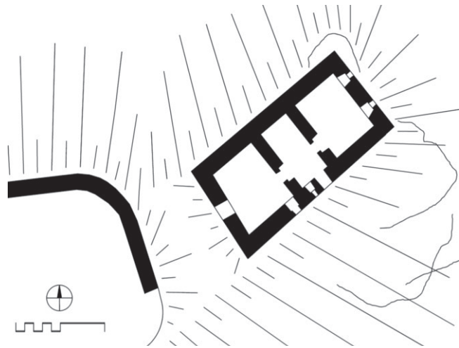
Moosham, Unterburg
